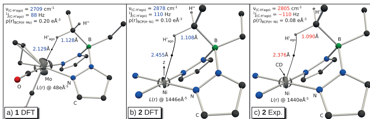
Figure 3. Theoretical and experimental L(r) = -\nabla^2\rho(r) isocontour surface maps of complexes a) 1 and b,c) 2 . Only bond paths between the individual metal and agostic hydrogen ( \text{H}'_{\text{ago}} ) atoms are drawn.
