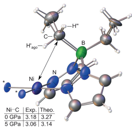
Figure 1. Overlay of structural fragments of 2 obtained by experimental X-ray diffraction studies at 0.0 and 5.0 GPa pressure using a diamond anvil cell (DAC); ellipsoids are set at 50% probability. For two of the nitrogen atoms (marked by *) only the ellipsoids at 5 GPa were drawn to illustrate the significant reduction of thermal motion in 2 at elevated pressures. Values of the Ni...C distances are given in Å.
